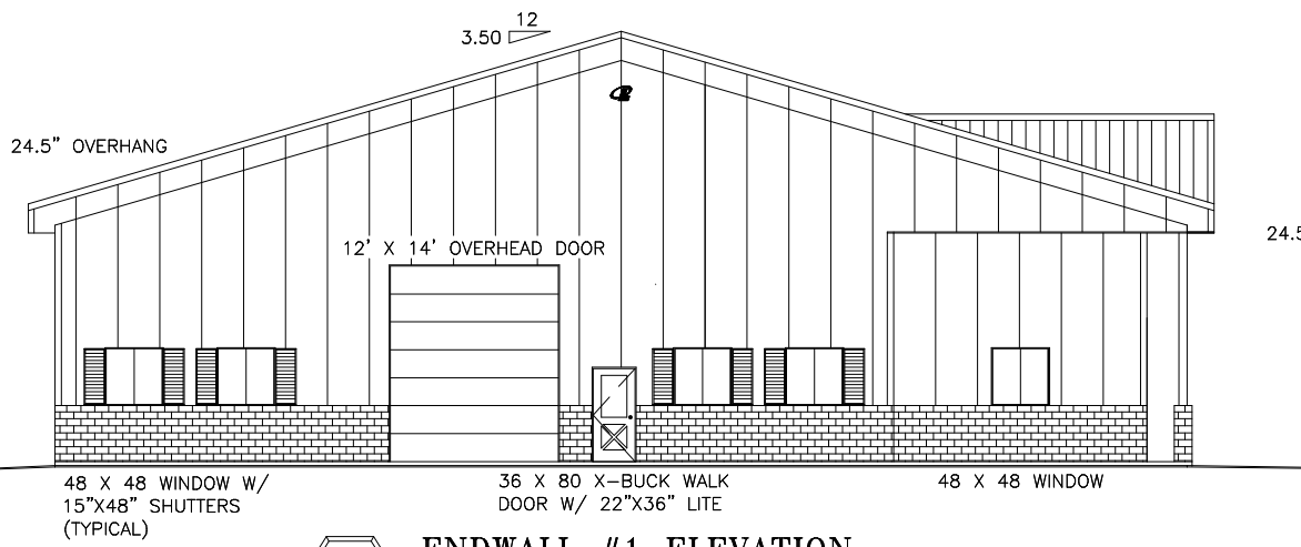
C16 ENDWALL #1 ELEVATION SCALE: 1/16=1
