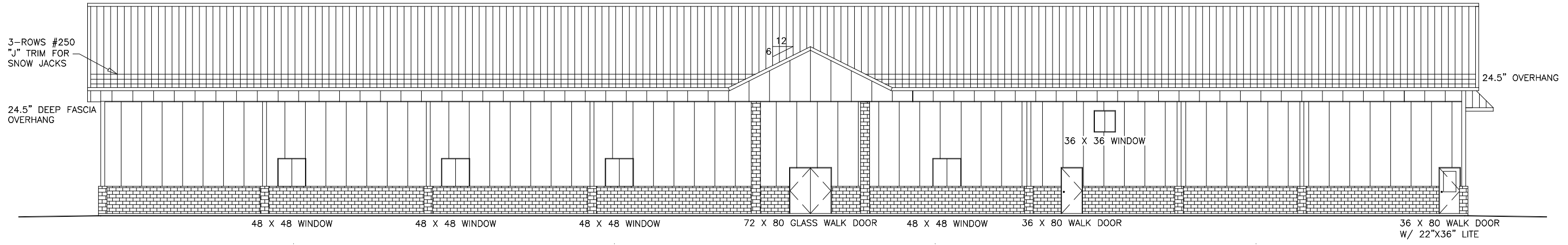
A16 SIDWALL #1 ELEVATION SCALE: 1/16=1
